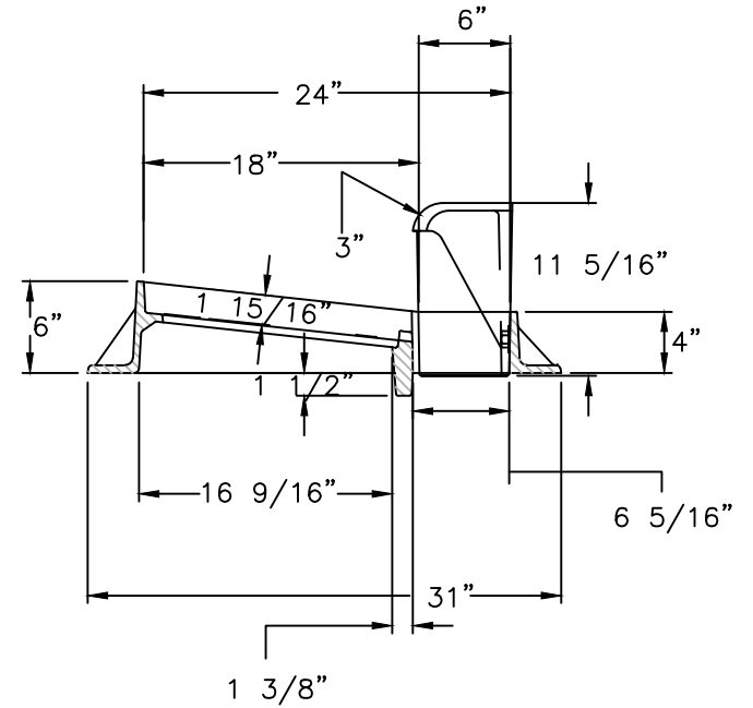
FRAME SECTION
